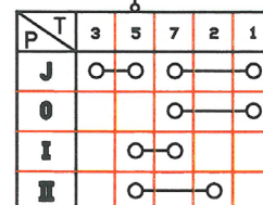
Wiper Switch
